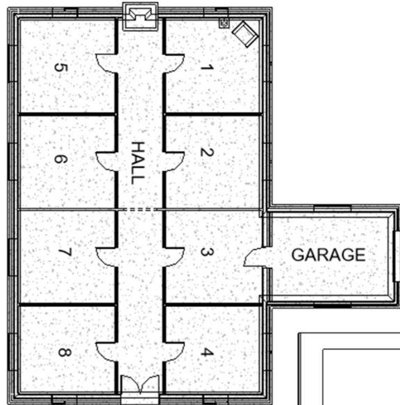
1 st Story Floor Plan
